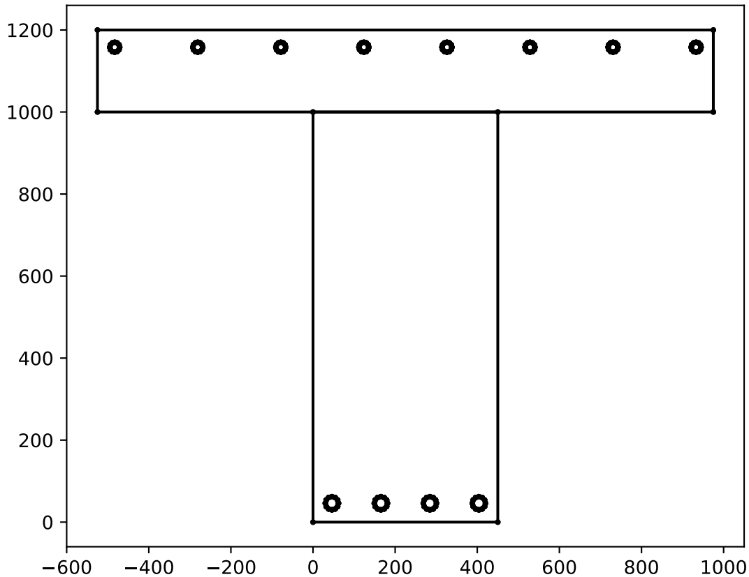
Cross-Section Geometry
