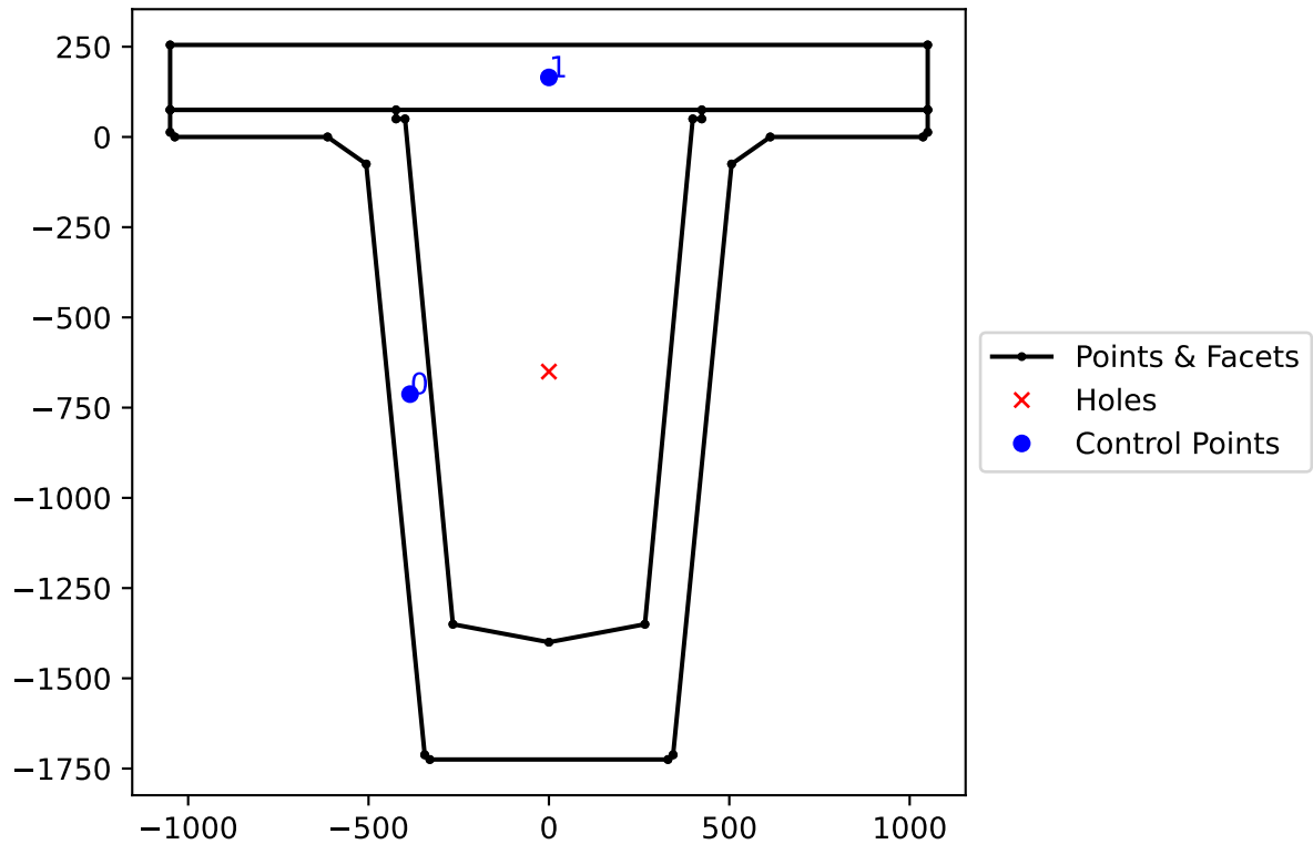
Cross-Section Geometry
