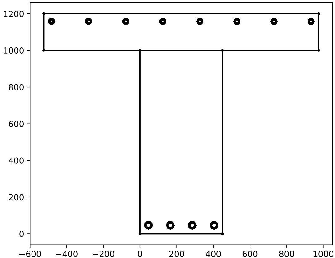
Cross-Section Geometry
