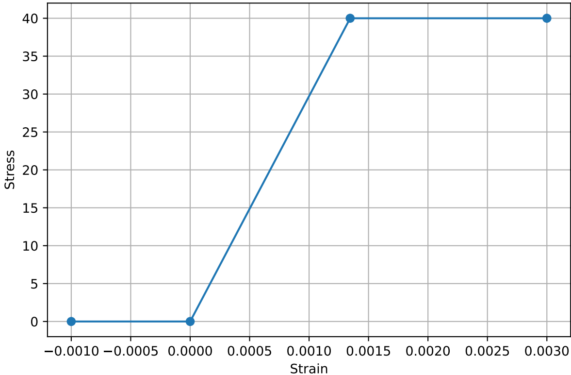
40 MPa Conc [2300 kg/m 3 ] (NZS3101:2006) - Service Profile
