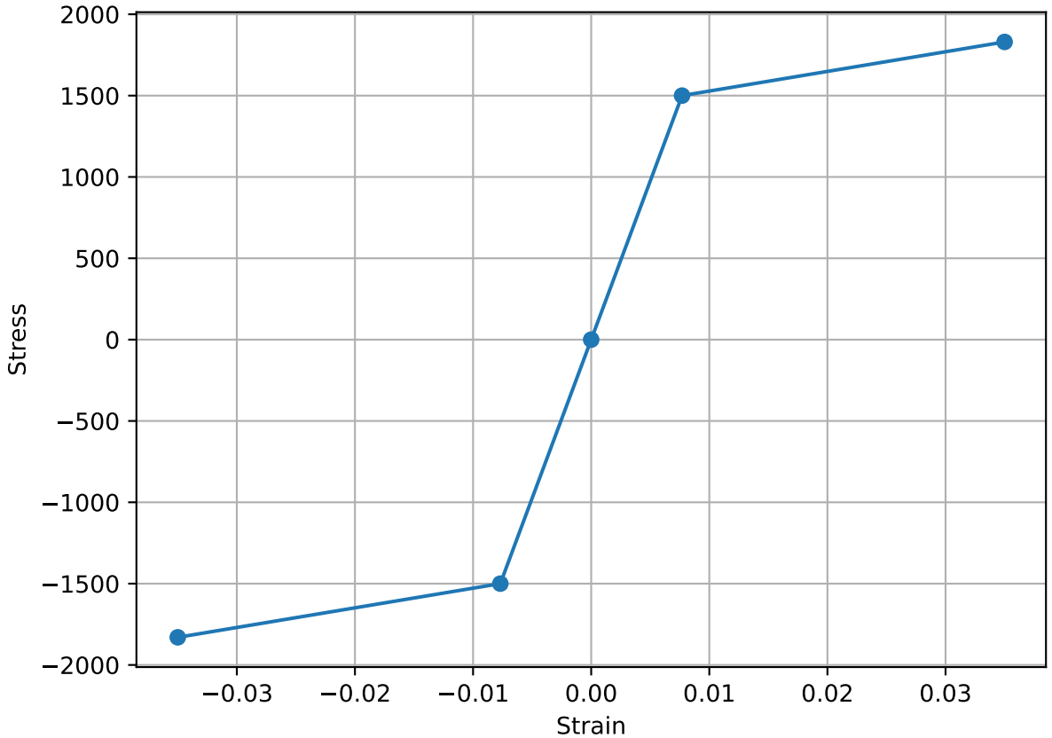
Stress-Strain Profile
